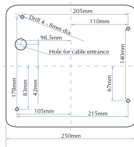
INSTALLATION TEMPLATE
